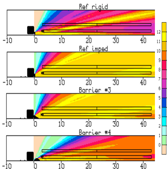
Figure 13: Tram (close track). Vertical maps of IL_A . From top to bottom: ref. and abs. barrier, Conf.3, Conf.4
