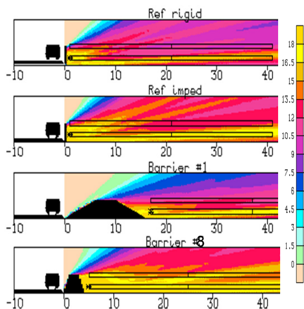
Figure 18: High speed train. Vertical maps of IL_A . From top to bottom: ref. and abs. barrier, Conf.1, Conf.8
