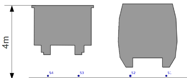
Figure 7: Geometry for the freight train (left) and high speed train (right)
