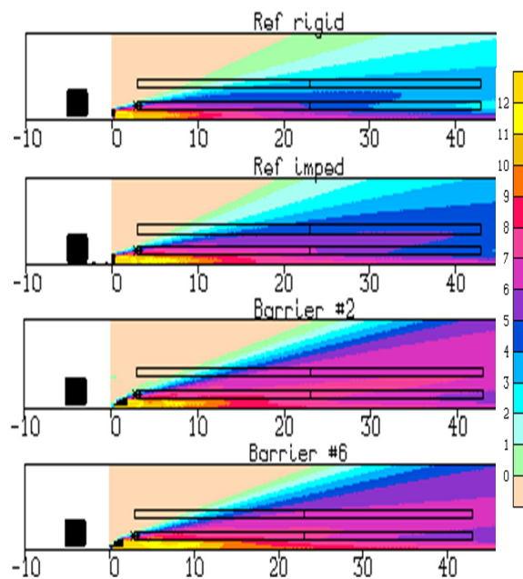
Figure 14: Tram (opposite track). Vertical maps of IL_A . From top to bottom: ref. and abs. barrier, Conf.2, Conf.6
