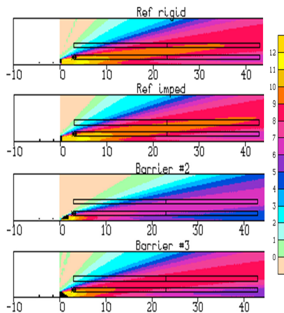
Figure 12: Cars in city center. Vertical maps of IL_A . From top to bottom: ref. and abs. barrier, Conf.2, Conf.3
