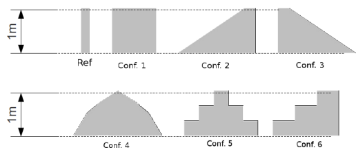
Figure 11: Geometry of low-height berms for city centers
