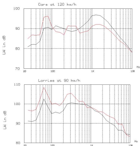
Figure 6: Power spectra for cars driving at 120 km/h (top) and lorries driving at 90 km/h (bottom). Rolling noise (black) and engine noise (red)
