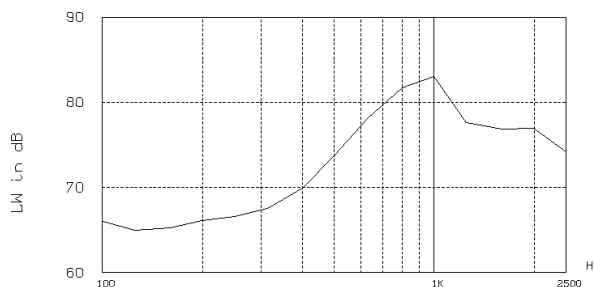
Figure 4: Power spectrum for the tram running at 30 km/h
