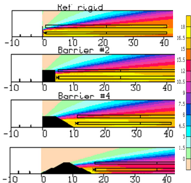
Figure 16: Motorway. Vertical maps of IL_A (From top to bottom: ref. barrier, Conf.2, Conf.4, Conf.6)
