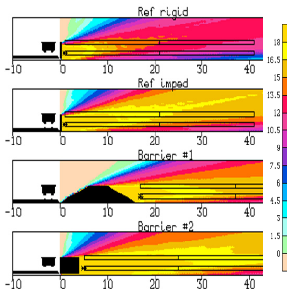
Figure 17: Freight train. Vertical maps of IL_A (From top to bottom: ref. and abs. barrier, Conf.1, Conf.2)
