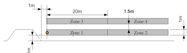
Figure 10: Definition of the 4 receivers' zones and the "pavement" receiver (circle)
