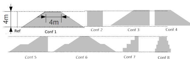
Figure 15: Geometry of berms along motorways
