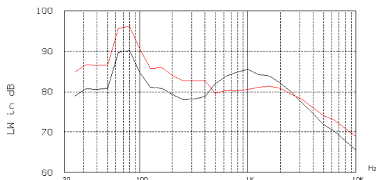
Figure 2: Power spectra for cars driving at 50 km/h. Rolling noise (black) and engine noise (red)
