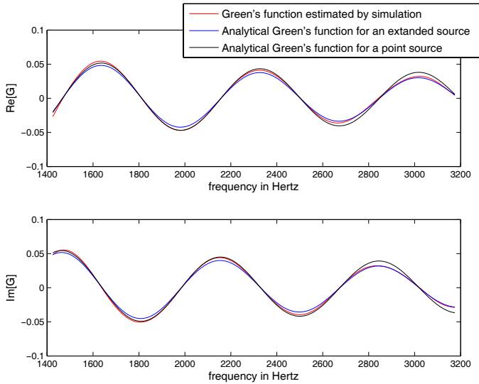
FIGURE 5 – Green's function G_{11} between the source m = 1 and receiver n = 1
