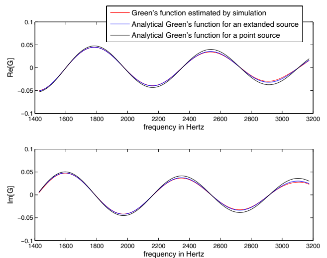
FIGURE 8 – Green's function G_{11} between the source m = 1 and the receiver n = 1
