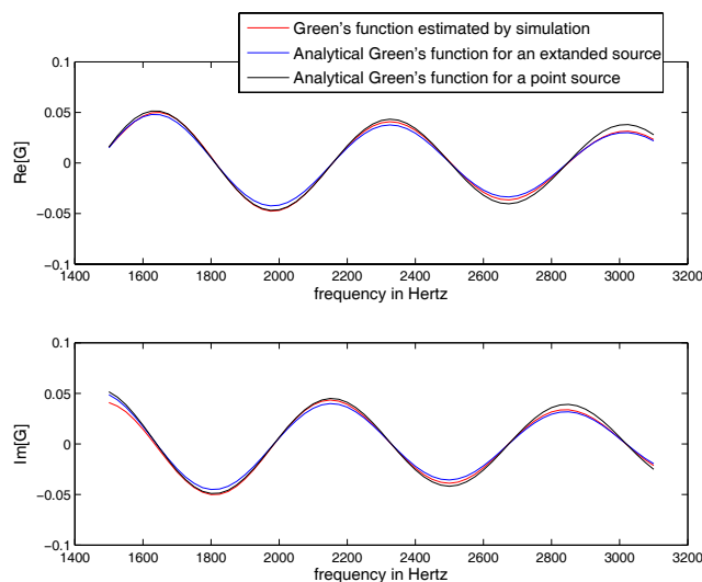
FIGURE 3 – Results obtained for the estimation of the Green's function between a source and a receiver placed at a distance R = 0.48
