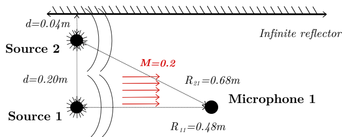
FIGURE 9 – Propagation of two sources in uniform flow M = 0.2 in the direction \vec{x}_1 in the presence of an infinite reflector
