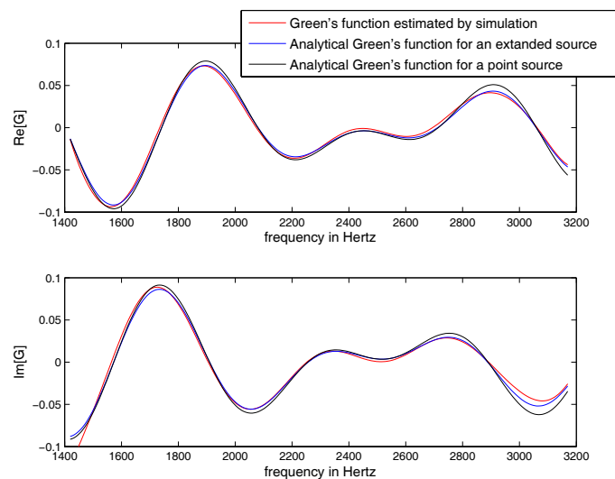
FIGURE 10 – Green's function G_{11} between the source m = 1 and the receiver n = 1 , in presence of a uniform flow and of a reflector
