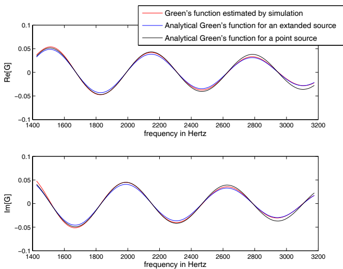
FIGURE 6 – Green's function G_{21} between the source m = 2 and receiver n = 1
