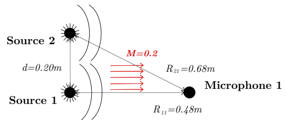
FIGURE 7 – Propagation of two sources in uniform flow M = 0.2 in the direction \vec{x}_1
