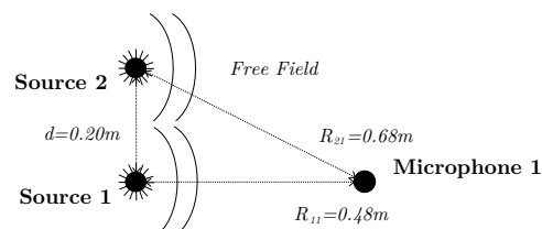
FIGURE 4 – Propagation in free field of two sources to a receiver to the respective distances R_{11} = 0.48 and R_{21} = 0.67
