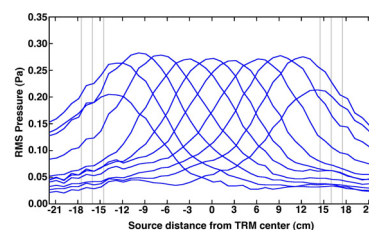
Figure 5: Source localization using TR-FSM imaging - Blue line: RMS pressure obtained after back-propagation for several source positions - Vertical gray lines: indicative radii of TRM layers
