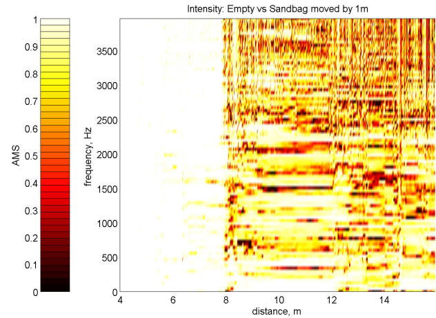
Figure 10: The ambiguity surface calculate for a 14.8m clay pipe with a blockage at 8m.
