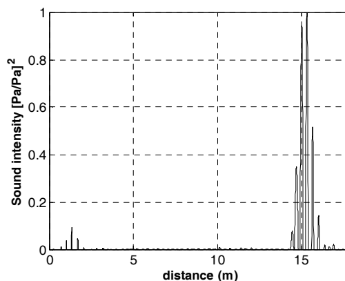
Figure 3: The positive intensity response for a clean, 14.8m long pipe with 150mm diameter (150-300 Hz range).
