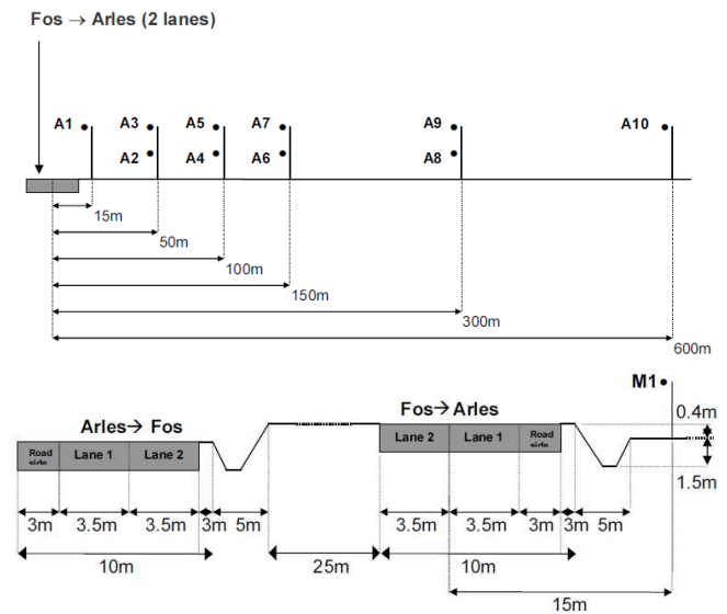
Figure 6: La Crau site (receivers heights : 1.5m and 4m). Receiver positions (top) and road description (bottom).
