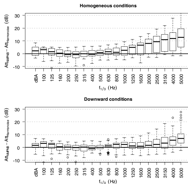
Figure 8: Boxplots of deviations between attenuations calculated with NMPB and with Harmonoise (all sites). Homogeneous (top) and downward conditions (bottom)
