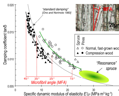
Figure 4: Relationship between axial \tan\delta and E'/\rho and principal affecting factors: slow-growth “resonance spruce” has a very low microfibril angle leading to very high E'/\rho and relatively low \tan\delta . Compression wood has a very high MFA and therefore low E'/\rho , but its more condensed lignin reduces its \tan\delta . Redrawn from [11].
