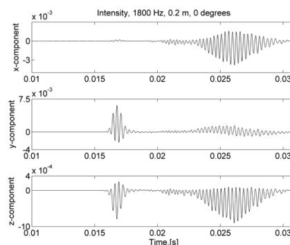
Figure 7: Intensity time history at 1800 Hz, 0.2 m, 0 degrees
