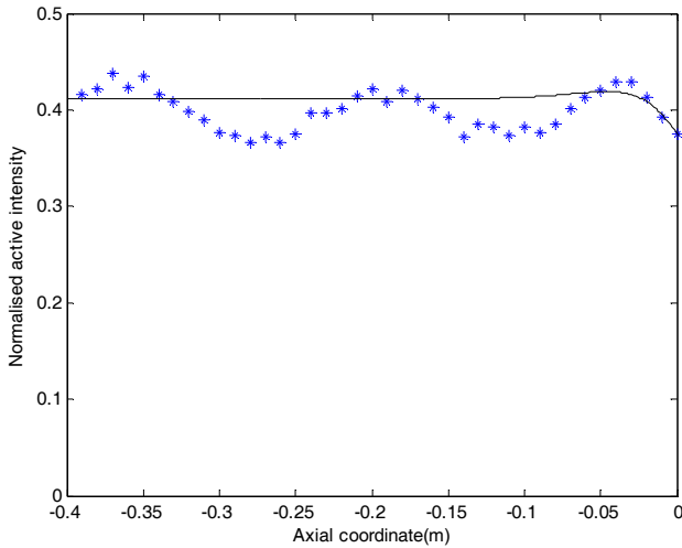
Figure 4: Time independent active intensity — theory; * * * * * , measurement.
