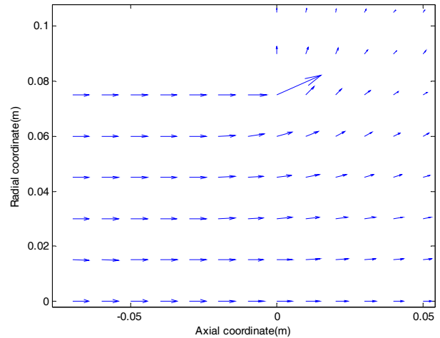
Figure 6: Time-independent active intensity distribution at 1 kHz
