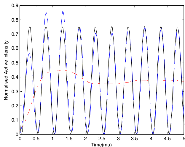
Figure 2: Instantaneous active intensity at 1kHz.
