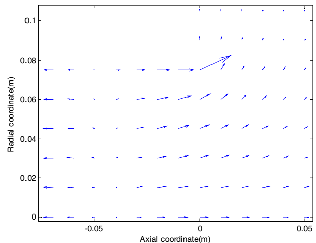
Figure 7: Time-independent reactive intensity distribution at 1 kHz
