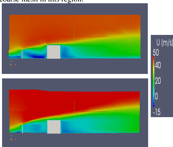
Figure 6 : mean longitudinal velocity in PIV plane, top LaBS, bottom measurement
