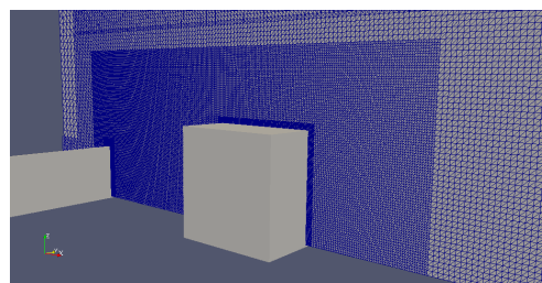
Figure 4 : mesh near to the geometry
