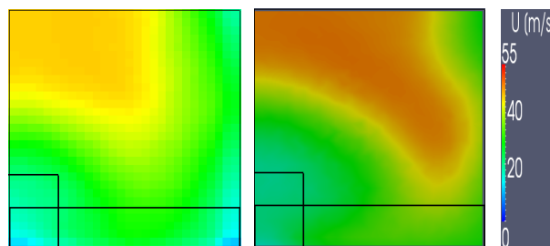
Figure 8 : mean longitudinal velocity in FC12h plane, left LaBS, right measurement
