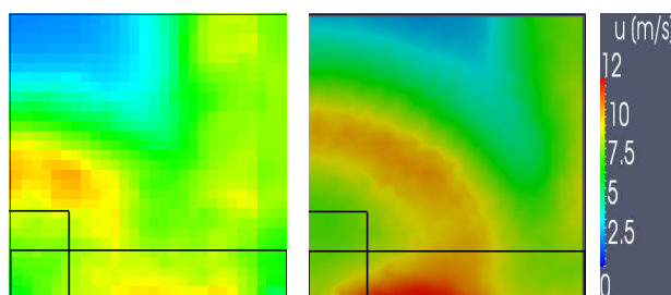
Figure 9 : fluctuating longitudinal velocity in FC12h plane, left LaBS, right measurement
