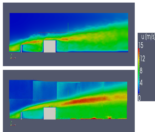
Figure 7 : fluctuating longitudinal velocity in PIV plane, top LaBS, bottom measurement
