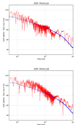
Figure 10 : PSD of wall pressure at points 14 and 15. Red LaBS, blue measurement
