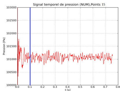
Figure 5 : simulation convergence
