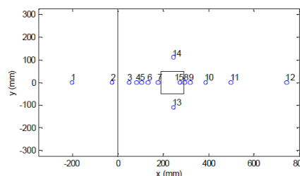
Figure 3 : Positions of wall pressure measurement points
