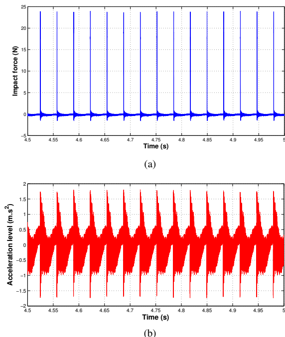
Figure 6: Third periodic orbit (1,1): (a) impact amplitude; (b) rigid support acceleration
