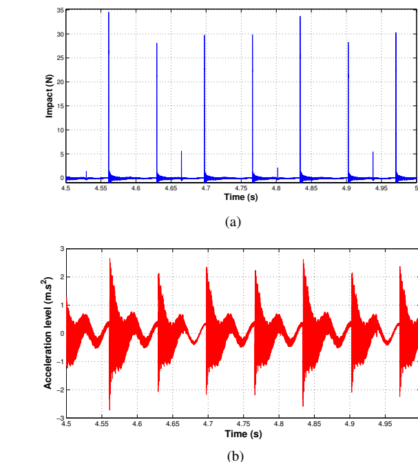
Figure 5: Second periodic orbit (6,8): (a) impact amplitude; (b) rigid support acceleration
