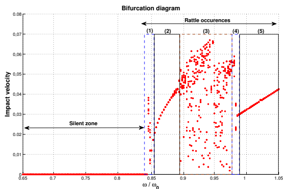
Figure 8: Numerical bifurcation diagram with a clearance of 0.045mm
