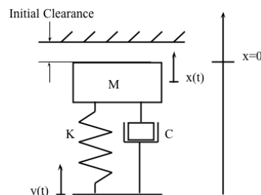
Figure 7: One degree of freedom impact oscillator
