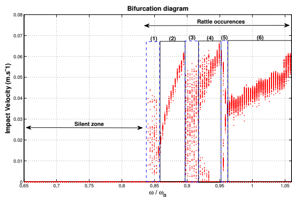
Figure 2: Experimental bifurcation diagram with presence of initial clearance
