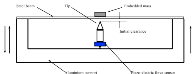
Figure 1: Experimental set-up
