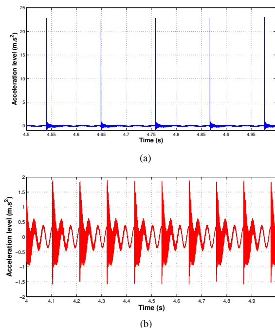
Figure 4: First periodic orbit (1,3): (a) impact amplitude; (b) rigid support acceleration
