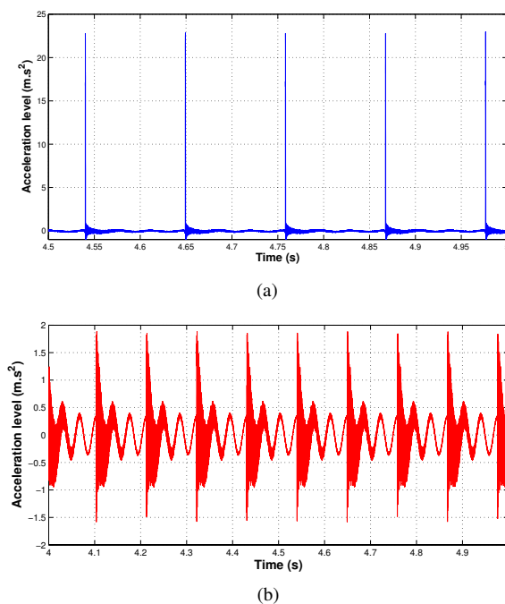
Figure 4: First periodic orbit (1,3): (a) impact amplitude; (b) rigid support acceleration
