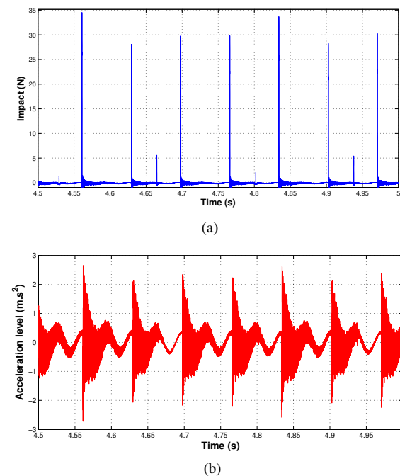
Figure 5: Second periodic orbit (6,8): (a) impact amplitude; (b) rigid support acceleration
