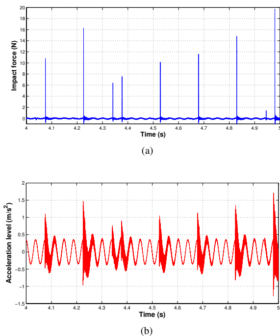
Figure 3: Apparent chaotic behaviour: (a) impact amplitude; (b) rigid support acceleration
