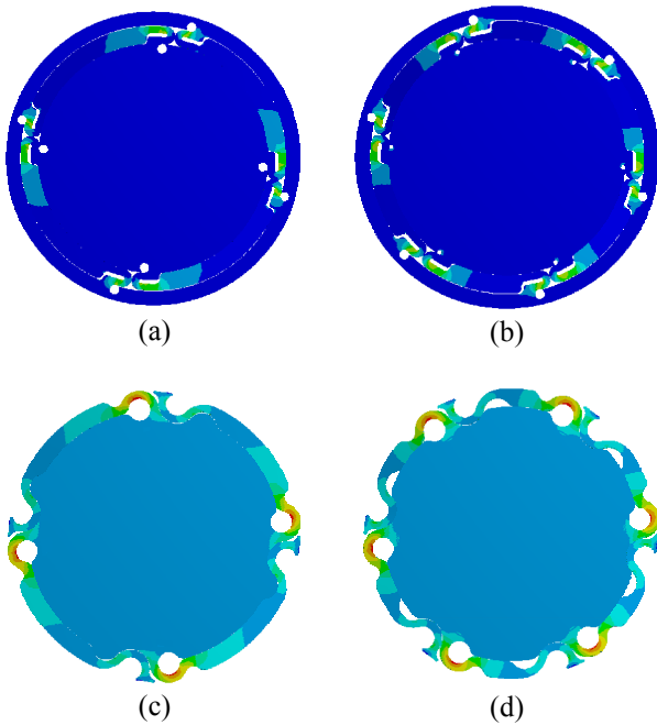
Figure 4: Stress distribution in the four suspension structures, for 300 μm out-of-plane displacement
