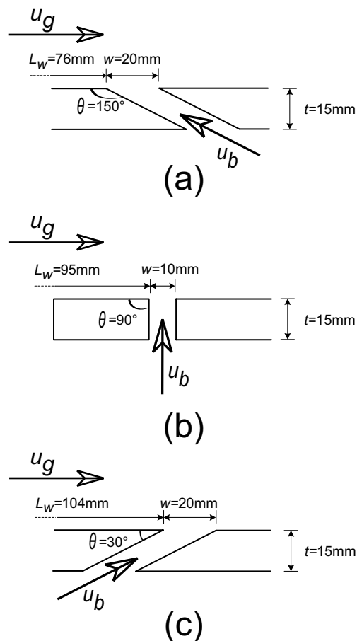
Figure 2: Schematic presentation of the three perforations: (a) perforation oblique in grazing flow direction ( \theta = 150^\circ ), (b) perforation with orthogonal edges ( \theta = 90^\circ ) and (c) perforation oblique in opposite grazing flow direction ( \theta = 30^\circ ). The arrow with subscript u_g indicate the grazing flow direction, the arrow with subscript u_b the bias outflow direction. Bias inflow is directed opposite to the bias outflow.
