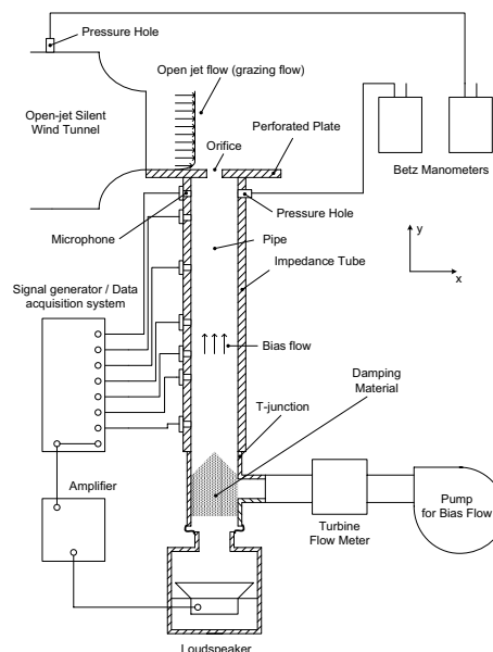
Figure 1: Schematic layout of the impedance tube setup.
