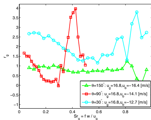
Figure 4: Grazing/bias inflow: acoustic perforation resistance r_g for the perforations having different angle of perforation: \theta = 150^\circ with |u_b|/u_g = 0.98 , \theta = 90^\circ with |u_b|/u_g = 0.84 and \theta = 30^\circ with |u_b|/u_g = 0.76 .
