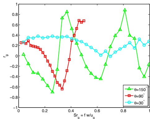
Figure 3: Pure grazing flow: acoustic perforation resistance r_g for the perforations with an obtuse upstream angle ( \theta = 150^\circ ), orthogonal edges ( \theta = 90^\circ ) and an acute upstream angle ( \theta = 30^\circ ). The grazing flow velocity is u_g = 16.8 m/s outside the boundary layer.
