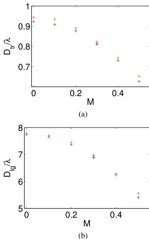
Figure 8: Medium in a uniform flow: (a) transverse resolution and (b) longitudinal resolution as functions of the Mach number for R_0/\lambda = L/\lambda = 15.5 . Black crosses refers to theoretical results and red crosses correspond to simulations results.
