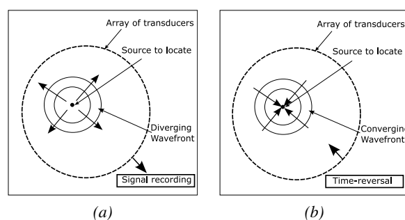
Figure 1: (a) First step of time-reversal: recording (b) Second step of time-reversal: re-emission
