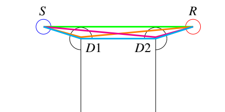
Figure 2: The diffraction edges ( D1, D2 ) create a volume around the edge which is non blocking. When a ray intersects only the first face, the path which can be found is S-R (green) and S-D1-D2-R (blue). When all intersections before a blocking face are allowed, the four diffracted paths are found. This strategy is used with NMPB08.
