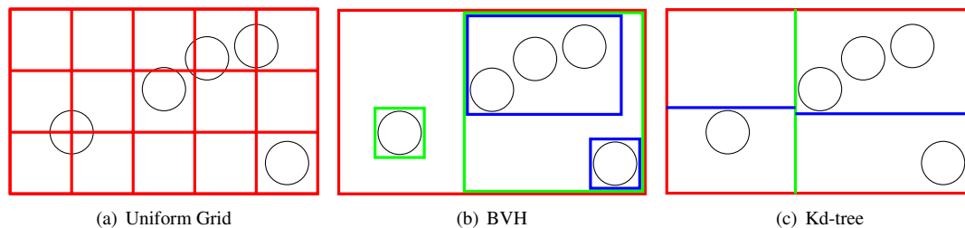
Figure 1: Example of a scene subdivide by a Uniform Grid, BVH and a Kd-tree. In a Uniform Grid (a), all the nodes are on the same level. For (b) and (c), the red node correspond to the root level of the hierarchy, the green nodes correspond to the level 1 and the blue nodes correspond to the level 2.
