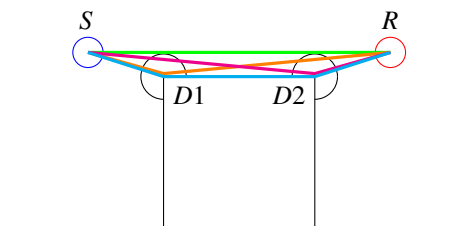
Figure 2: The diffraction edges ( D1, D2 ) create a volume around the edge which is non blocking. When a ray intersects only the first face, the path which can be found is S-R (green) and S- D1 - D2 -R (blue). When all intersections before a blocking face are allowed, the four diffracted paths are found. This strategy is used with NMPB08.
