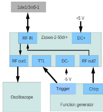
Figure 12: Sensors (1dw1r3m5-1) remote interrogation principle
