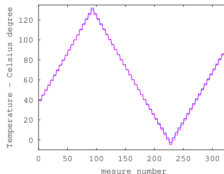
Figure 11: Magenta curve is for an oven reference sensor, blue curve corresponds to the sensors prototype.
