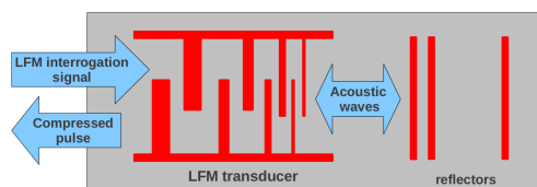
Figure 5: One port device prototype.
