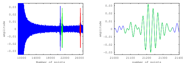
Figure 9: The three pulses: green colour marks is the second pulse, red- the third pulse
