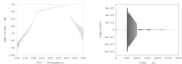
Figure 6: Extraction of the signal generated by the LFM transducer
