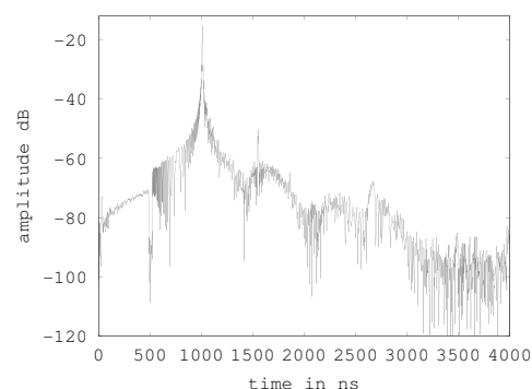
Figure 8: Compressed pulse with dB scale
