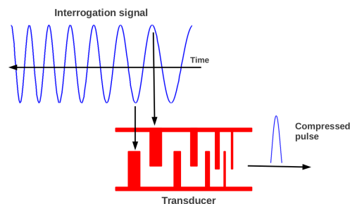
Figure 3: The interrogation signal compresses by IDT.
