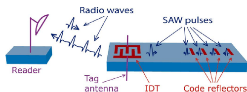
Figure 1: Operating principle of SAW RFID tag ( Ref: unknown source ).
