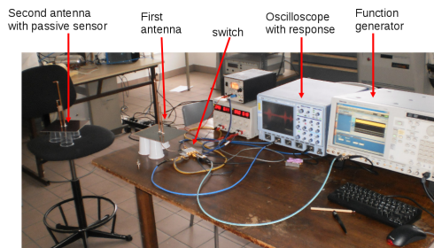
Figure 13: Remote interrogation
