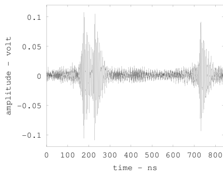
Figure 14: Remote interrogation - response pulses
