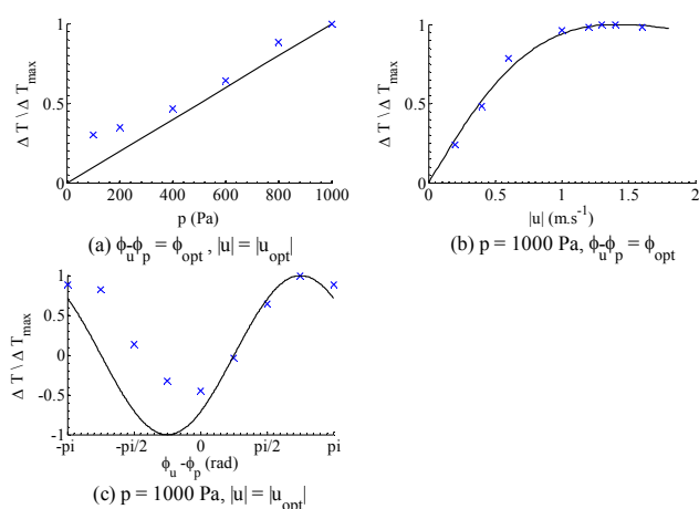
Figure 2: Normalized temperature difference \Delta T / \Delta T_{max} between the stack ends measured ( \times ) and calculated (solid line) as a function of (a) the acoustic pressure p , (b) the particle velocity amplitude u and (c) the phase \varphi between the particle velocity and acoustic pressure.
