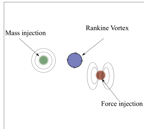
Figure 1: Schematization of the cases used to illustrate the method of complex variables. The aeroacoustic field is composed by two acoustic sources, and a Rankine vortex.
