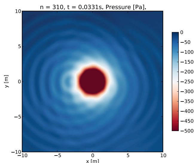
Figure 2: Total fluctuating pressure field.
