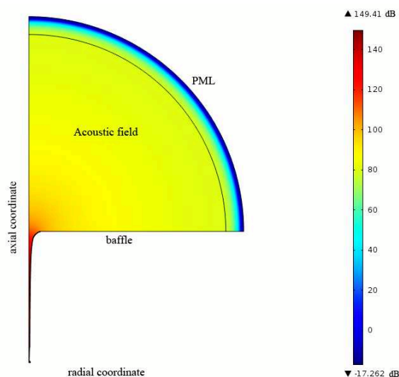
Figure 6: Acoustic pressure field of a straight trumpet bell at 440 Hz, modelled using a two-dimensional axisymmetric geometry.
