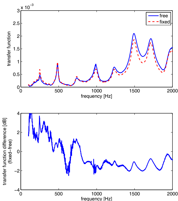
Figure 5: (top) Transfer function of a straight bell measured 1 m away from the bell as a function of frequency, for the case of a free vibrating bell (blue) and a heavily damped bell (red dashed). (bottom) Difference in the transfer functions caused by damping the bell.
