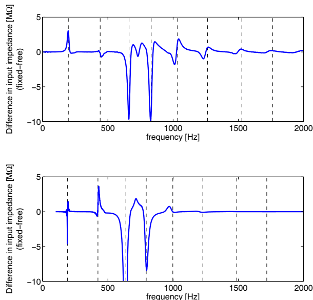
Figure 9: Difference in the input impedance of the bell caused by the wall vibrations measured experimentally (top) and calculated numerically (bottom). The dashed lines indicate the locations of the impedance peaks.
