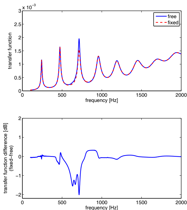
Figure 7: (top) Simulated transfer function of a straight bell calculated 1 m away from the bell as a function of frequency, for the case of a free vibrating bell (blue) and a fixed bell (red dashed). (bottom) Difference in the transfer functions caused by fixing the bell.
