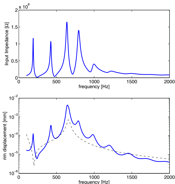
Figure 8: Input impedance of the free vibrating bell (top) and rim displacement caused by a vibrating piston excitation of the air column (bottom). The dashed curve shows the mechanical resonance of the bell (rim displacement caused by a structural acceleration at the mouthpiece).
