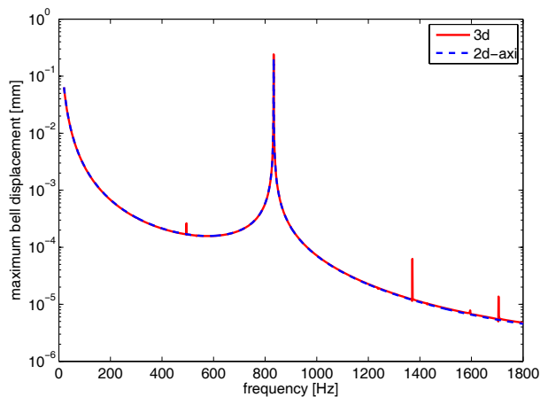
Figure 1: Maximum bell displacement over frequency stimulated by a force applied at the mouthpiece, as calculated using a 2d axisymmetric and a 3d model.
