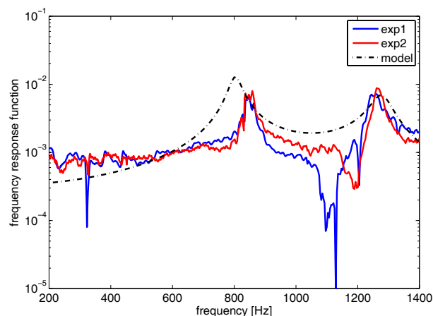
Figure 4: Frequency response function (average rim displacement relative to mouthpiece displacement) measured on a straight bell and calculated using the mass-spring model presented in [10].
