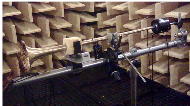
Figure 3: Experimental setup to measure the vibrations of the straight bell.
