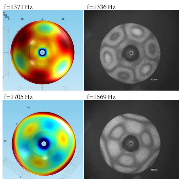
Figure 2: Elliptic modes of the vibration of the trumpet bell, as calculated from a 3D simulation (left) and observed using electronic speckle pattern interferometry (right).
