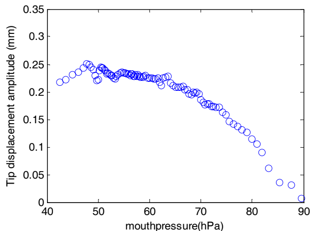
Figure 3: reed tip displacement amplitude versus mouthpressure (measurement).
