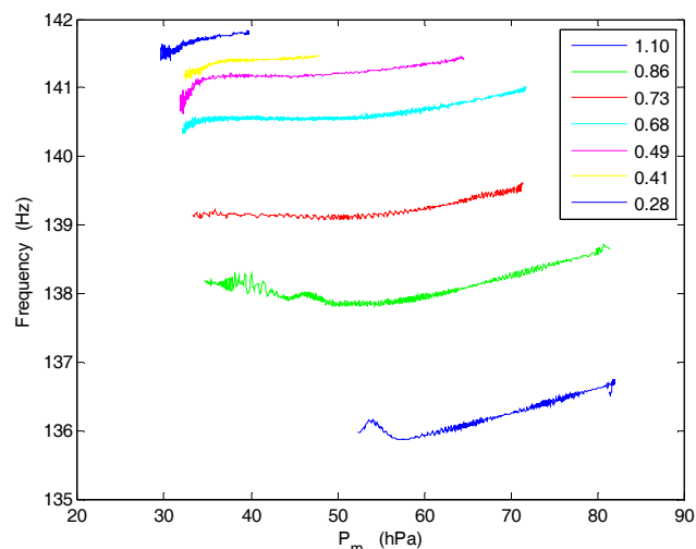
Figure 4: Playing frequency versus mouthpressure for various reed opening (from 1.1mm to .28mm from bottom to top).
