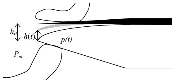
Figure 1: Schematic view of a clarinet mouthpiece and notations
