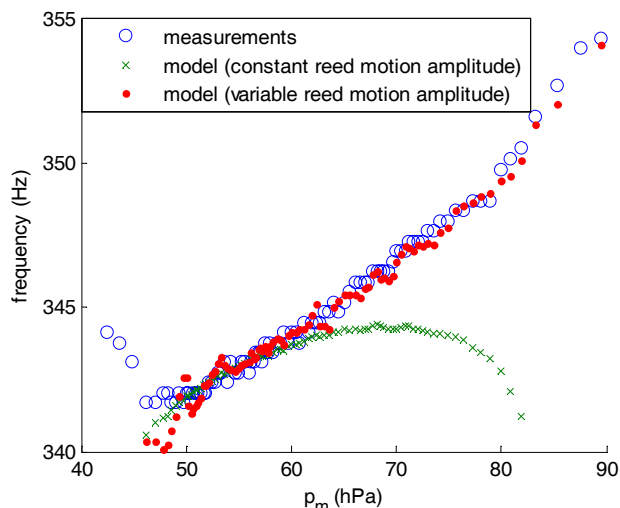
Figure 2: Playing frequency versus mouthpressure for a given embouchure.
