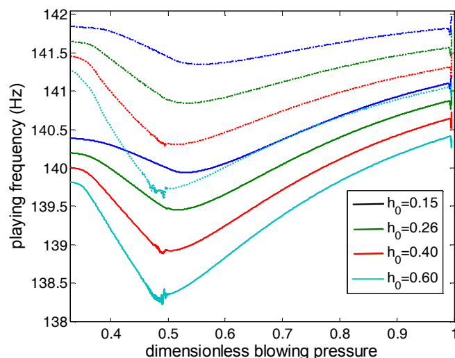
Figure 4: Playing frequency versus dimensionless blowing pressure P_m/P_M for various reed opening h_0 (mm).
