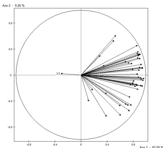
Figure 5: Principal component analysis.
