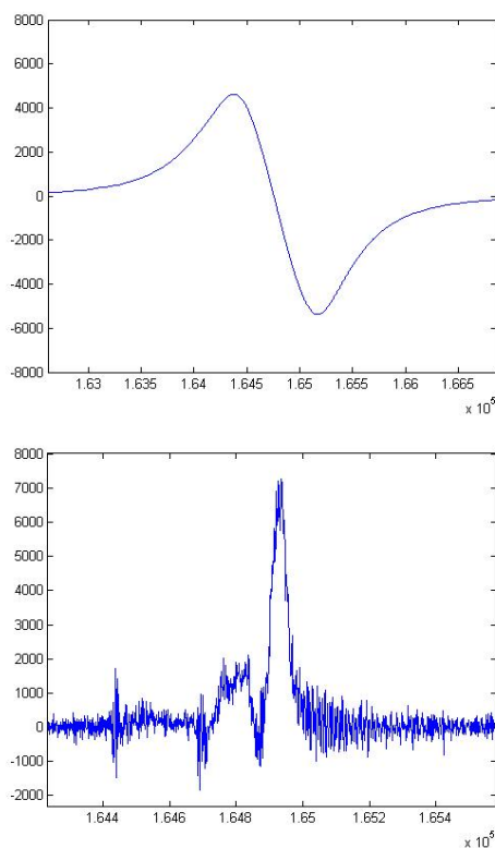
Figure 2: Compression component (top) and residual part (bottom) of the elementary cylinder pressure derivative.
