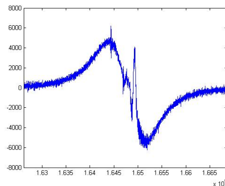
Figure 1: Example of one temporal derivation of in-cylinder pressure signal, focused near the auto-ignition process.
