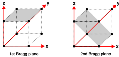
Figure 2: The first and second Bragg planes of a 3-D square lattice.
