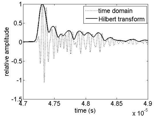
Figure 6: Time domain signal of the wave transmitted through sample 1 and its Hilbert transform.
