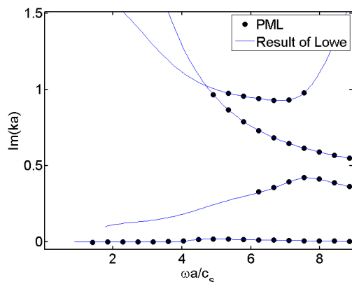
Figure 3: Im(ka) vs. dimensionless frequency for alpha-titanium
