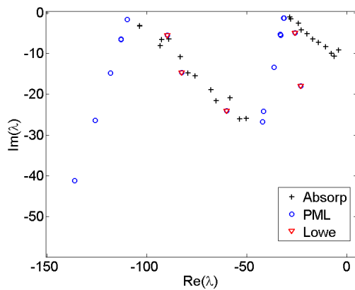
Figure 6: Same as Fig. 5 at \omega a/c_s = 9.498 .
