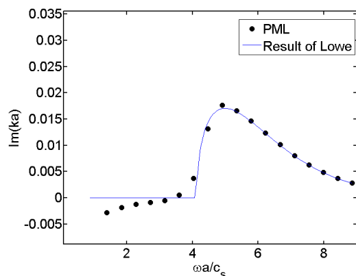
Figure 4: Same as Fig. 3. Zoom on the less attenuated mode.
