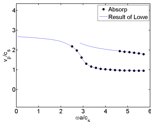
Figure 7: Dimensionless phase velocity v_p/c_s vs. frequency for epoxy-aluminium.
