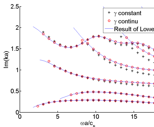
Figure 2: Im(ka) vs. dimensionless frequency for titanium-alpha-titanium. Comparison between \gamma constant and parabolic.
