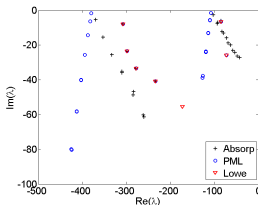
Figure 5: Spectrum of \lambda = -k^2 in the complex plane at \omega a / c_s = 17.68 (titanium-alpha-titanium).
