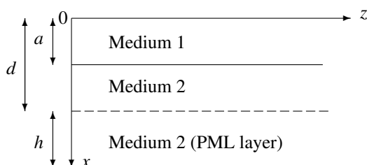
Figure 1: Geometry of a bilayer waveguide with PML in the transverse direction. With a SAFE method, only the x direction needs to be discretized.
