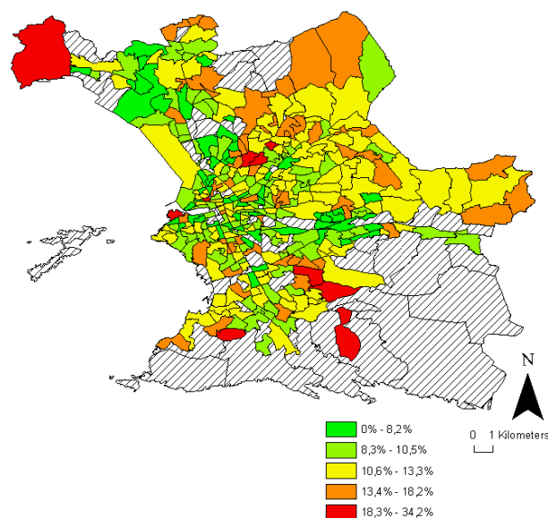
Figure 2: Spatial variability of potential noise exposure on road traffic L_{den} (%)
