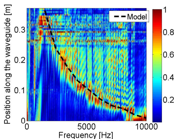
Figure 10: Experimental tonotopic map obtained by taking the normalized response for each frequency. Map for the plate immersed in the air.
