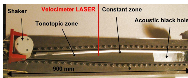
Figure 6: Annotated photography of the assembled experimental setup.
