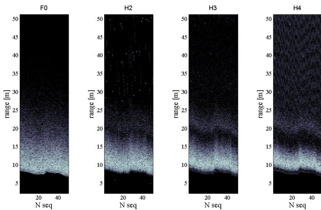
Figure 4. Waterfall of data along 50 pings (x axis) for the first four harmonics.
