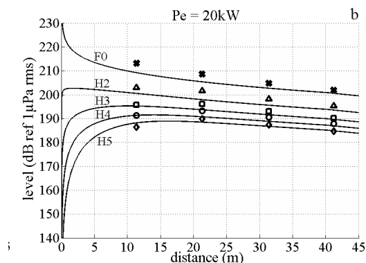
Figure 1. Harmonics level versus distance. P_e = 20 kW. Marks: measurements. Lines: pseudo-1D model.
