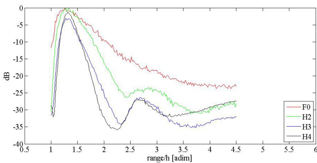
Figure 5. Mean harmonic response versus the ratio range/height, computed with the data displayed in Fig. 4.
