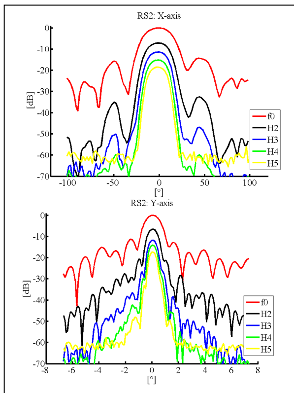
Figure 2. Directivity of the first harmonics ( z = 41 m, P_e = 20 kW). Top: x -axis. Bottom: y -axis
