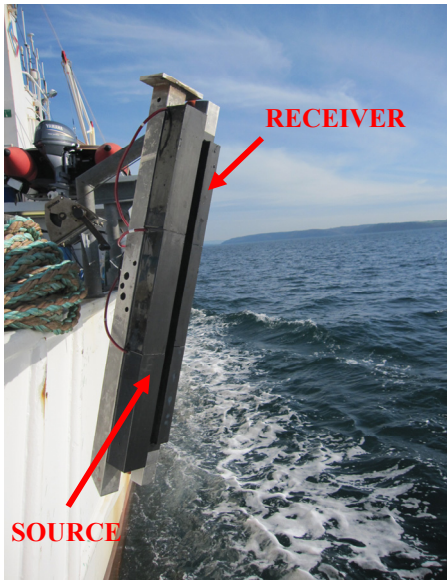
Figure 3. Multifrequency source and wideband receiver used during the sea trials in the bay of Brest.
