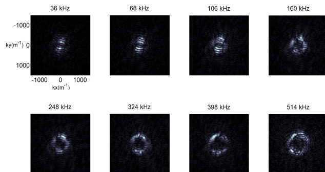
Figure 9: 3D Fourier transform in the range of [0\text{ kHz}-600\text{ kHz}] in the ring electrode case.
