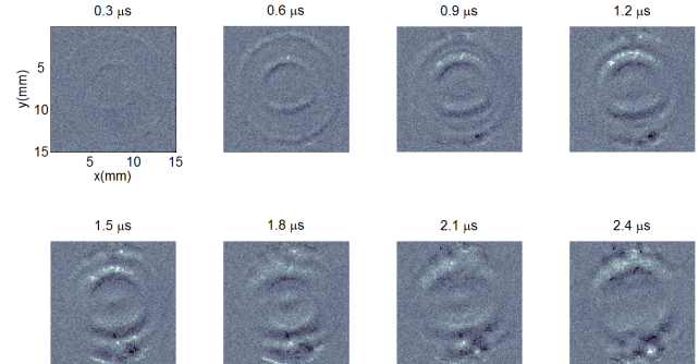
Figure 5: Space-time signals recorded for the sensor with ring geometry electrodes.
