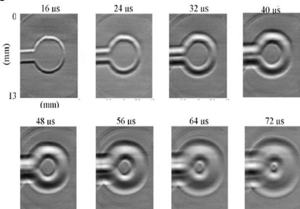
Figure 4: Space-time signals recorded for the sensor with disk geometry electrodes.
