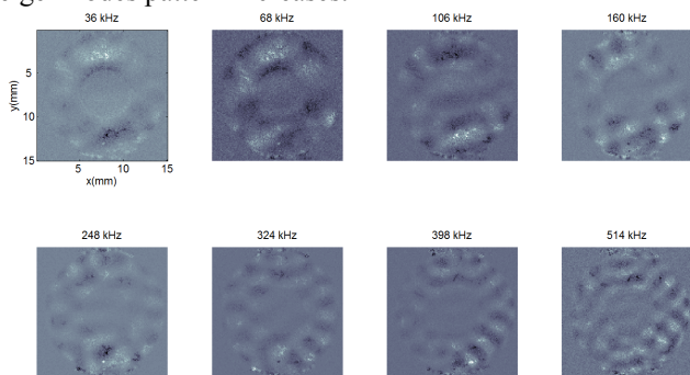
Figure 8: Time Fourier transform for identifying the wave modes in the ring electrode case.
