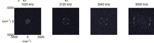
Figure 10: 3D Fourier transform in the range of [1\text{MHz}-9\text{MHz}] in the ring electrode case.
