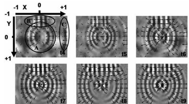
Figure 6: Gabor analysis of the disk electrodes setup for F = 1 \text{ MHz} .
