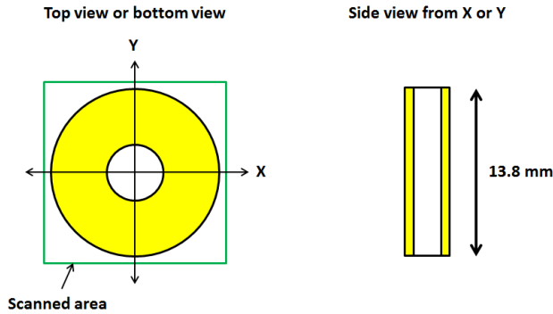
Figure 3: Geometry of the quartz and the electrodes used in the current experiment.
