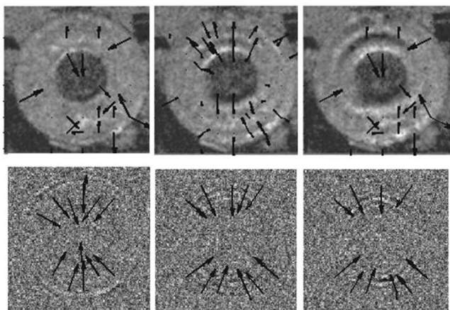
Figure 7: Gabor analysis of the ring electrodes setup. Upper for F=0.8\text{MHz} and from left to right for time 0\mu\text{s} , 1\mu\text{s} and 2\mu\text{s} . Lower for F=2.1\text{MHz} and from left to right for time 0\mu\text{s} , 1\mu\text{s} and 2\mu\text{s} .
