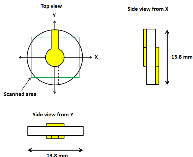
Figure 2: Geometry of the quartz and the electrodes used in the classical experiment [1-2].
