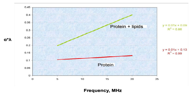
Figure 4: Frequency dependences of absorption coefficient.
