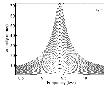
Figure 12: Plexiglass sample NRUS results
