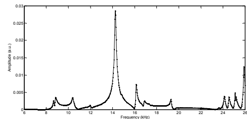
Figure 5: Resonance mode of a cylinder. (a) wavelength compared to the length of the sample. (b) resonance mode
