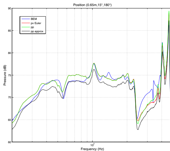
Figure 10: FSM and BEM pressures at the back of the subwoofer
