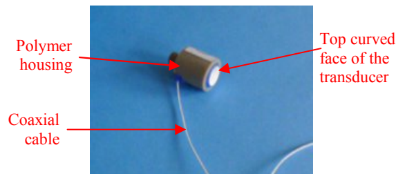
Figure 4: Photographs of the transducer.
