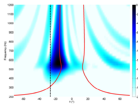
Figure 10: Detection of the direction of arrival for the rail model. The excitation is located at -30° (black line) and the theoretical angle, \theta_0 , is in red.
