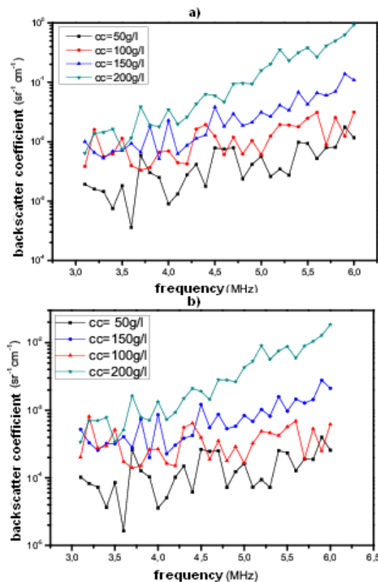
Figure 2: Experimental curves of the backscatter coefficient versus frequency around 5MHz for different graphite concentrations ( 50 g/l, 100 g/l, 150 g/l, 200g/l) obtained by using a) Sigelman and Reid method and b) Chen method.
