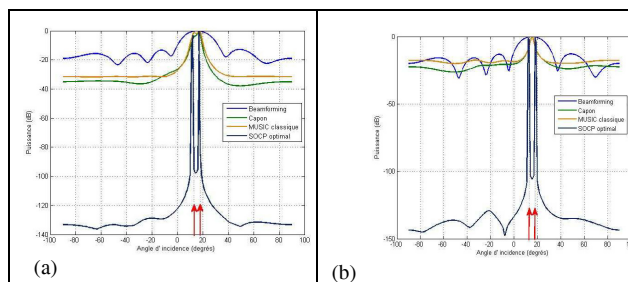
Figure 6 : Localization of acoustical sources in anechoic room. (a) Uncorrelated sources; (b) Correlated sources
