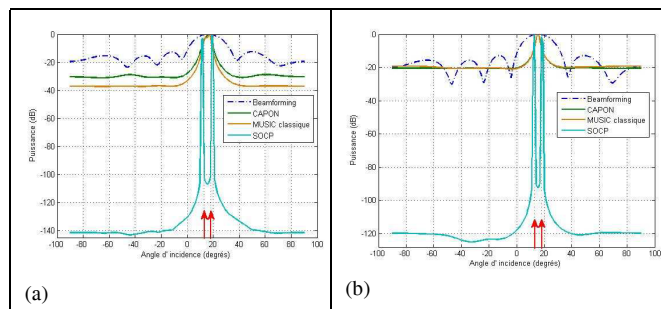
Figure 2 : (a) Localization of two uncorrelated sources ; (b) localization of two correlated sources
