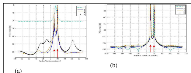
Figure 3 : Sensitivity of (a) MUSIC and (b) SOCP optimal to the assumed number of sources
