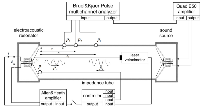
Figure 7: Schematics of the experimental setup.
