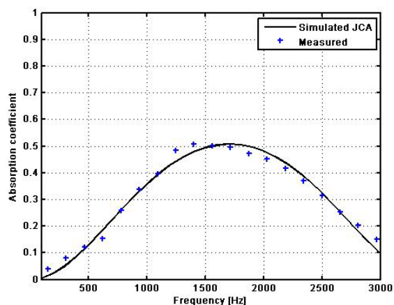
Figure 4. Absorption curve of a mesh with parameters ( d, t, p, Y_d, D ) = (36 \mu\text{m} , 50 \mu\text{m} , 28 %, 33 \mu\text{m} , 5cm).
