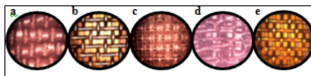
Figure 6. Microscopic image of the meshes tested a) Woven screen, b) sefar® acoustic BHY, c) sefar® Nitex 41/31, d) curtain e) sefar® acoustic HF 34-39.
