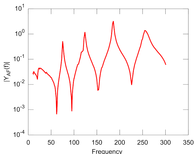
Figure 4: Frequency response of the joist-wood connector-beam system
