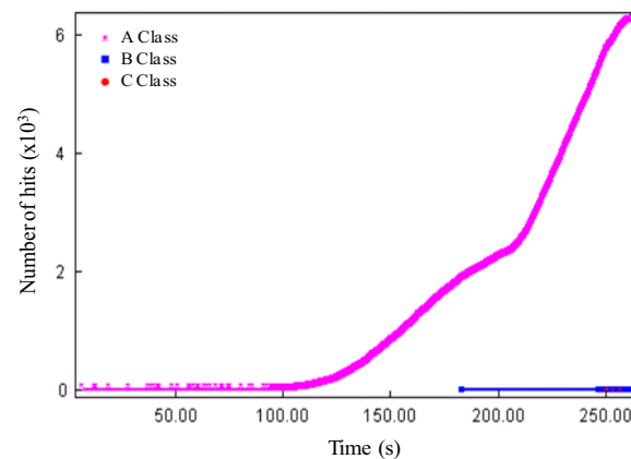
Figure 6. Time dependency of the identified damage mechanisms for specimen without integration (WS) in static test
