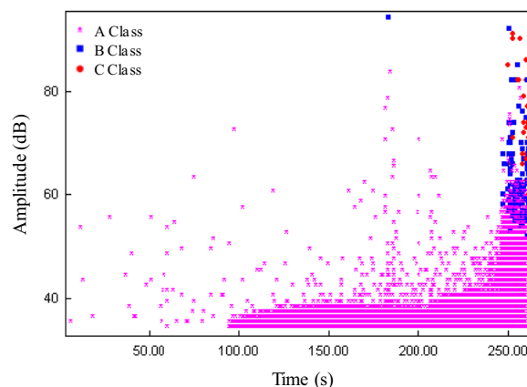
Figure 5. Distribution of amplitude vs time for specimen without integration (WS) in static test
