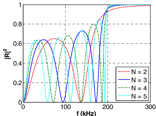
Figure 3: Comparison of the reflection spectrum of N \times (AI/PE) periodic structures.
