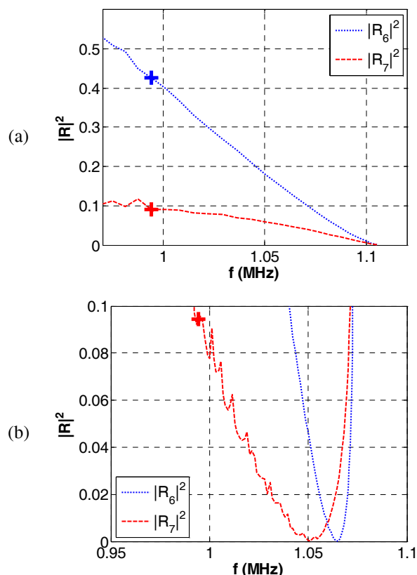
Figure 10: Copper defect layer insertion at locations 6 and 7 influence on the minimum of |R|^2 as a function of (a) thickness 0 < d_{\text{copper}} < 0.6 mm ('+' : d_{\text{copper}} = 0.5 mm), (b) density 1500 < \rho < 10000 kg/m 3 ('+' : \rho = 8900 kg/m 3 ).
