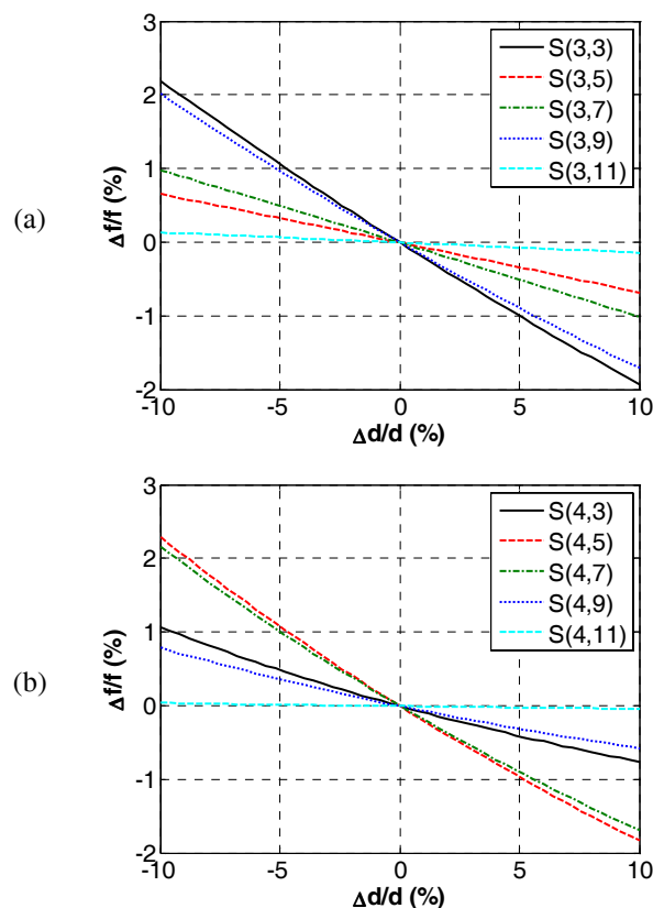
Figure 6: Sensitivities (a) S(3,n) for the mode VM_3 and (b) S(4,n) for the mode VM_4 , depending on the PE layers n = 3, 5, 7, 9, 11 .
