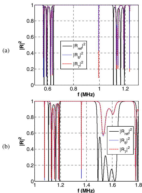
Figure 9: Reflection spectrum of the 5 \times (\text{Al/PE}) periodic structure with (a) copper and (b) glass defects inserted at locations 6 and 7.
