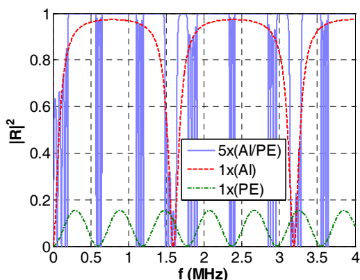
Figure 2: Reflection spectra of the 5x(AI/PE) periodic structure, of an Al plate and of a PE plate.
