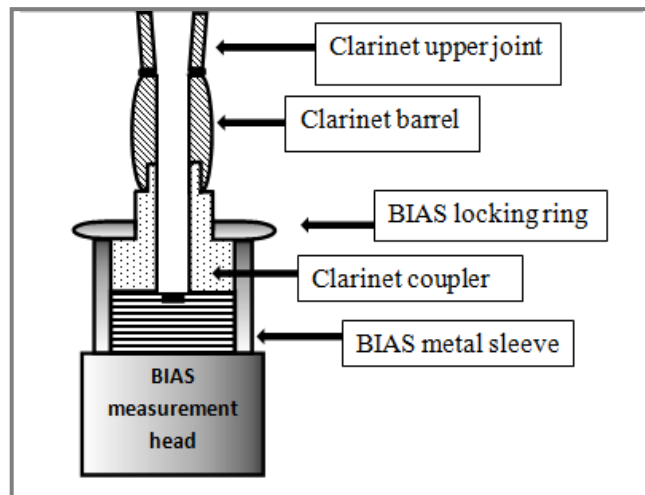
Figure 9: Schematic diagram of BIAS measurement head coupled to clarinet
