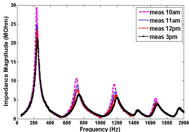
Figure 6: Impedance magnitude curves for Buffet B12 clarinet without mouthpiece; Bb3 fingering applied using putty/PTFE tape.
