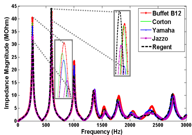
Figure 13: Impedance magnitude curves for five student model clarinets with E5 fingering applied.
