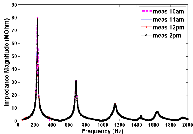
Figure 7: Impedance magnitude curves for Buffet B12 clarinet without mouthpiece; Bb3 fingering applied using small clamps.
