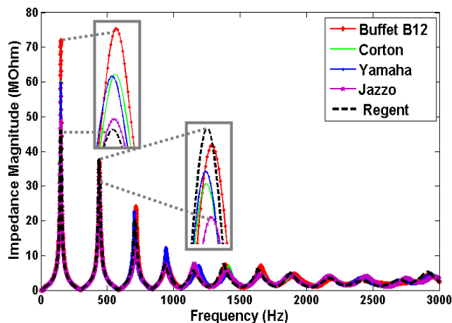
Figure 11: Impedance magnitude curves for five student model clarinets with E3 fingering applied.
