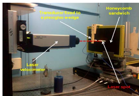
Figure 12: Experimental setup
