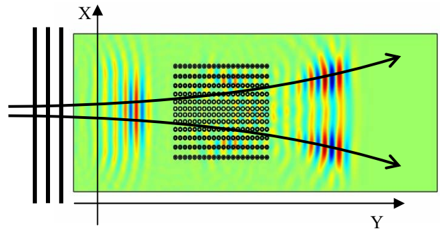
Figure 12: Simulation of the deviation at t = 560\mu s for ka = 0.85 , showing the reflected wave, the splitting of the transmitted wave and the trajectories.
