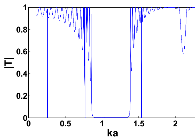
Figure 2: Transmission coefficient for 14 rows
