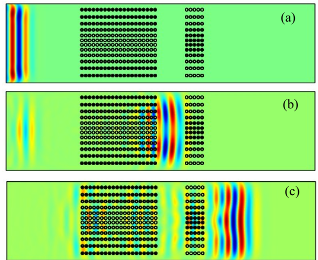
Figure 13 Simulation of the deviation and its rebuilding, at t=90\mu s (a), t= 471\mu s (b) and t= 636\mu s (c) for ka=0.64
