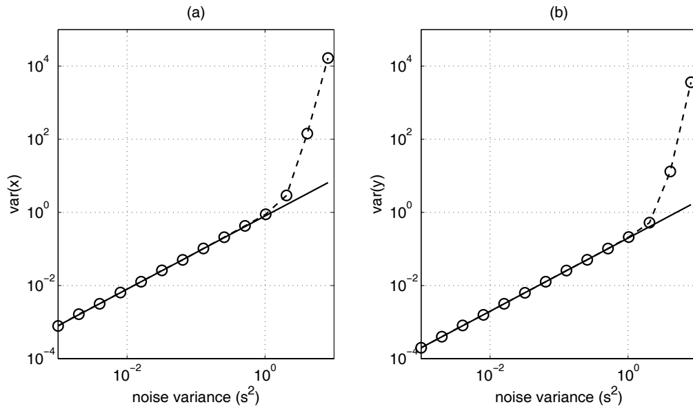
Figure 3: CRB(x) (a) and CRB(y) (b) versus variance of noise for the coordinate pair (x, y) = (4.5, 4.5) .
