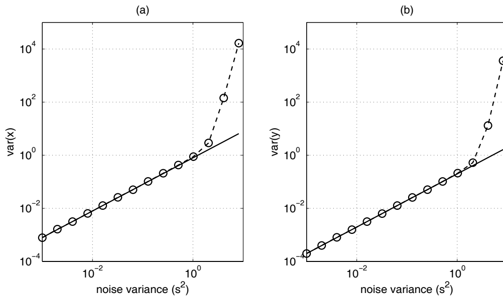
Figure 3: CRB(x) (a) and CRB(y) (b) versus variance of noise for the coordinate pair (x, y) = (4.5, 4.5) .
