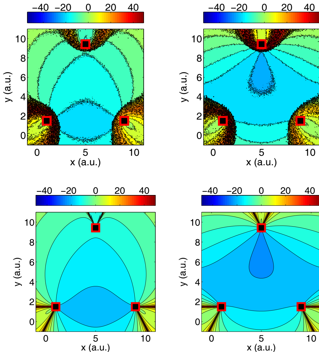
Figure 2: \text{var}(x) (upper left) - \text{var}(y) (upper right) - \text{CRB}(x) (down left) - \text{CRB}(y) (down right) .
