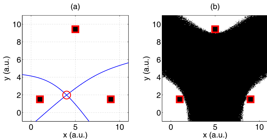
Figure 1: Location of the 3 sensors (ref. sensor at the top of the plate) (a) - Valid zone of measurement (black) (b).
