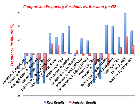
Figure 12: Comparison of Frequency Residuals ( \zeta ) vs. Bassoon for Raw and “Redesign” Data for Note G2. The raw or unmodified results are in blue, while the modified wing joint results are in red.
