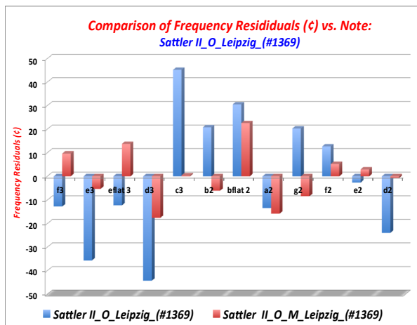
Figure 10: Comparison of Frequency Residuals ( \zeta ) vs. Note for “Redesign Results of the Sattler II_O_Leipzig (#1369). The raw or unmodified results are in blue, while the modified wing joint results are in red.
