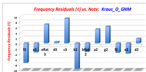
Figure 1: Frequency Residuals (¢) vs. Note for the original Kraus bassoon in the collection of the German National Museum (Kraus_O_GNM)
