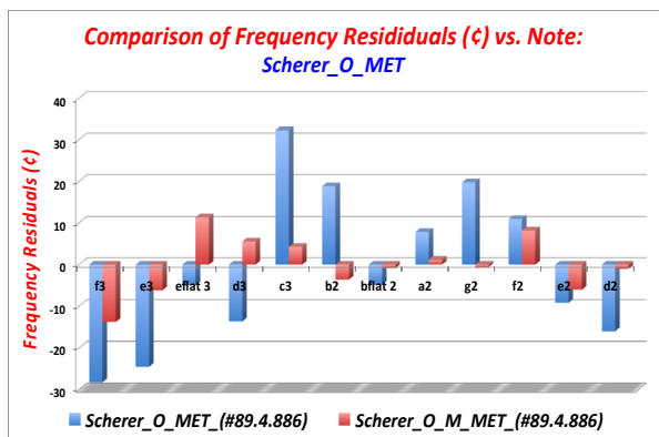
Figure 11: Comparison of Frequency Residuals ( \zeta ) vs. Note for “Redesign” Results of the Scherer_O_MET. The raw or unmodified results are in blue, while the modified wing joint results are in red.
