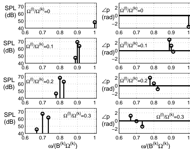
Figure 3: Acoustic pressure p_{\omega j}^{(k)←(l)} as a function of the dimensionless frequency \omega/(B^{(k)}\Omega^{(k)}) at \mathbf{x}_j = (R, \pi/4, 0) for \vec{F}_{n1} = [0.2N, 0.3N, 0.5N]^T \forall n \in [B - 1, B + 1] . Left: SPL, right: phase. Up to down : \Omega^{(l)}/\Omega^{(k)} = [0, 0.1, 0.2, 0.3] .
