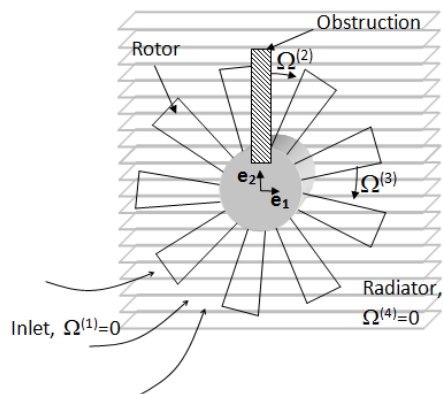
Figure 4: Multi-row configuration
