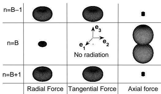
Figure 2: Simulated directivities from Eq. (10). Left to right: \vec{F}_{n1} = [1N, 0, 0]^T , \vec{F}_{n1} = [0, 1N, 0]^T , \vec{F}_{n1} = [0, 0, 1N]^T . Up to down: n = B - 1 , n = B , n = B + 1
