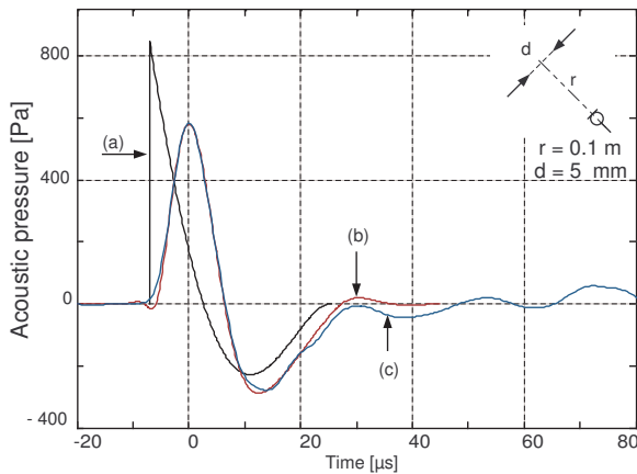
Figure 4: Acoustic pressures p(t) versus time. (a) Initial waveform (Eq. 1) with P_{Max} = 848.25 Pa , t_+ = 9.6 \mu s and \tau = 32.5 \mu s . (b) Effect of low pass filtering on Initial waveform (low-pass filter with cut-off frequency f_c = 62 kHz and attenuation 0.45 s ). (c) Measured pressure at r = 0.1 m of a spark discharge with d = 5 mm .
