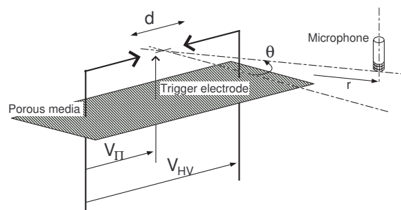
Figure 1: Schematic representation of a three-electrodes system for the generation of sparks and the experimental set-up used for the measurement of acoustic waveform. V_{II} and V_{HT} are the trigger voltage and the capacitor voltage; d and r are the gap length and the distance from the centre of the discharge.
