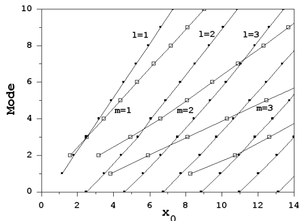
Figure 12. Regge trajectories of the first families of resonances for a QF20 porous cylinder with sealed pores. Empty boxes: m family. Filled boxes: l family.
